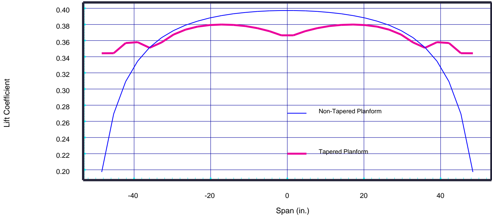
Lift Coefficient
