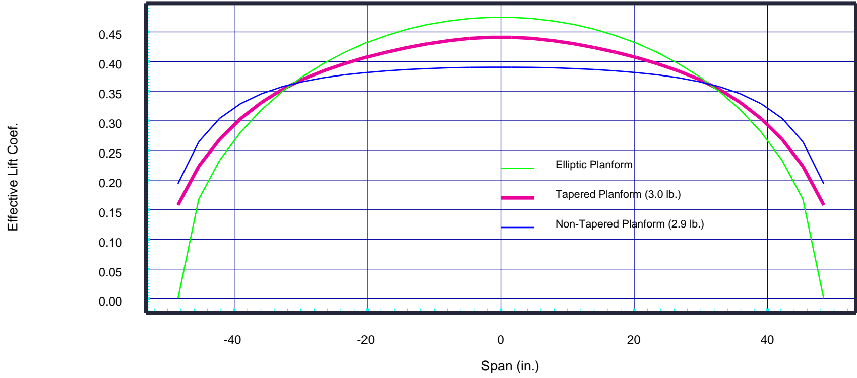
Lift Distribution
