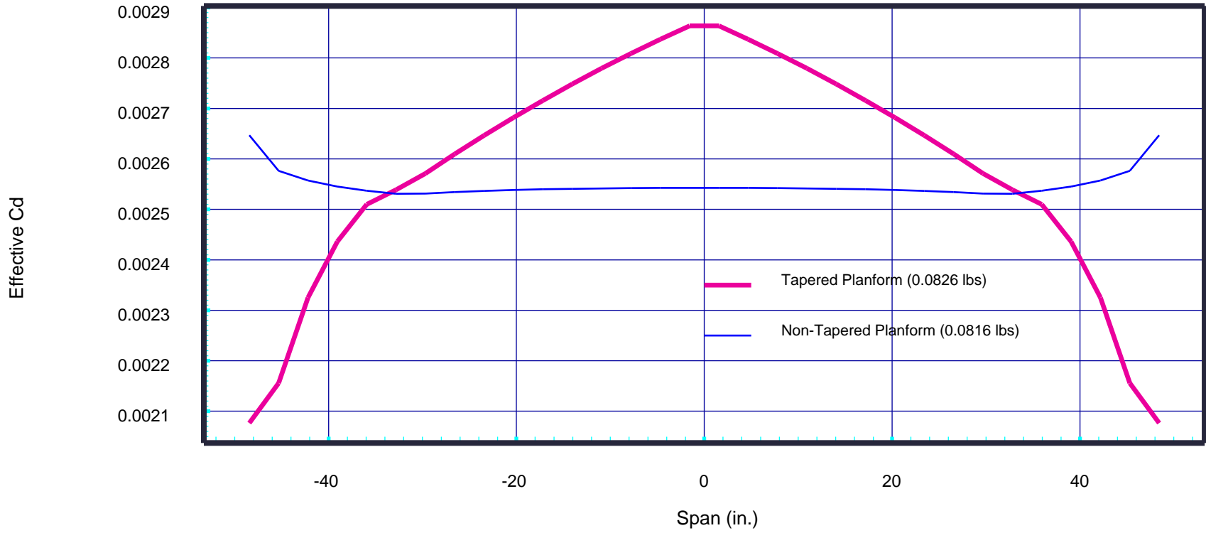
Drag Profile (SD7037 Airfoil)
