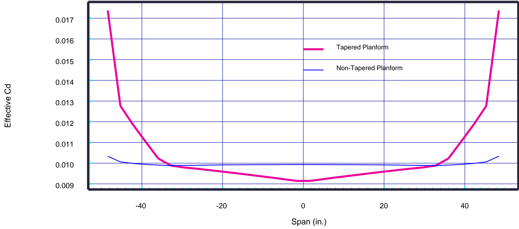
Drag Coefficient (SD7037 Airfoil)
